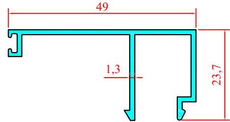
AS 01 6252 TEK CAM ÇITA PROF. 0.380 Kg/m
