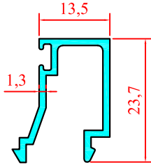
AS 01 6254 TEK CAM ÇITA PROF. 0.240 Kg/m
